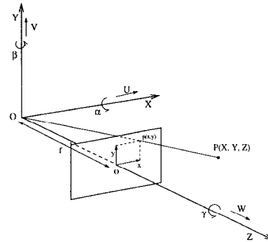
Figure 1. The camera coordinate system.
